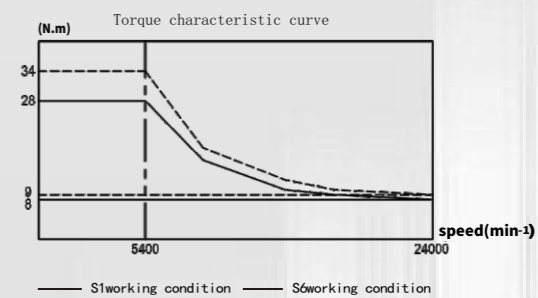
HSK E50 24000RPM 16/19KW 28/34Nm
